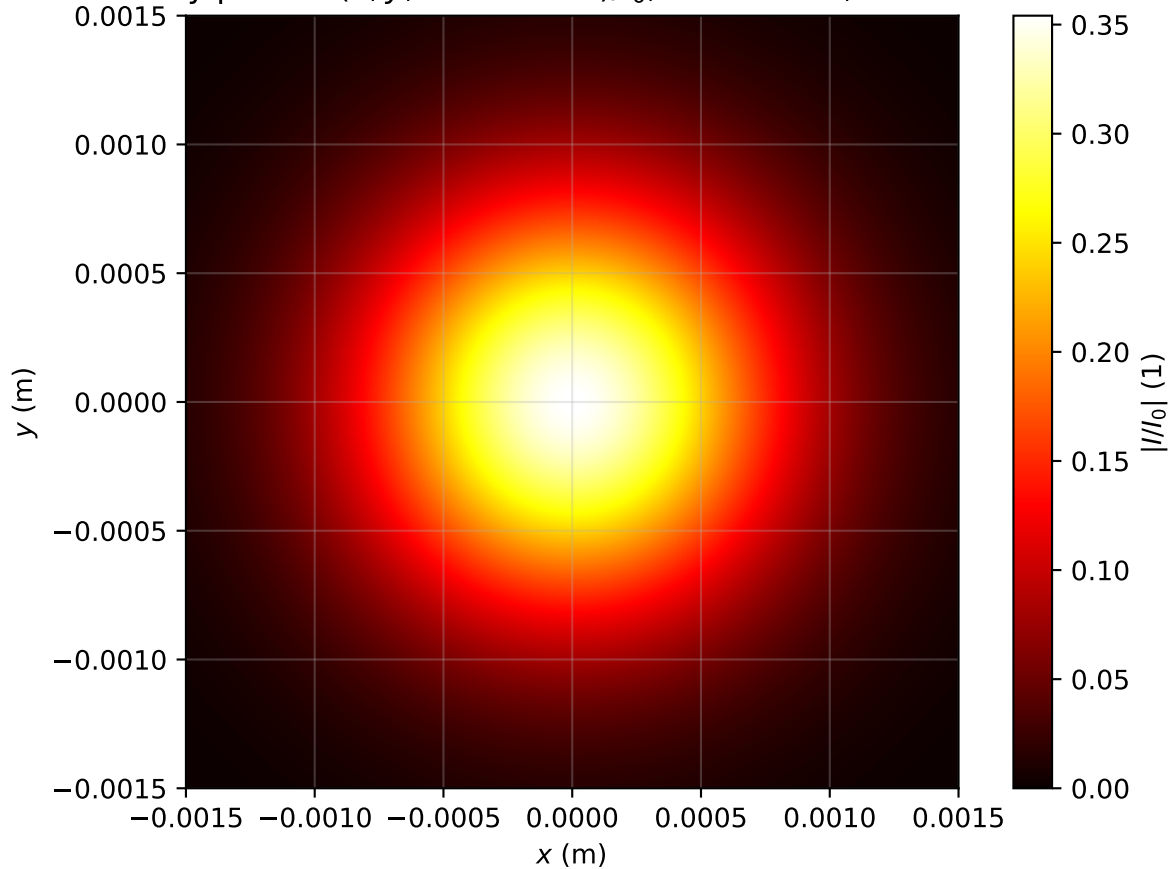
Intensity profile I(x, y, z = 3.423m)/I_0 , P_{in}=0.3P_{cr} , artificial time
